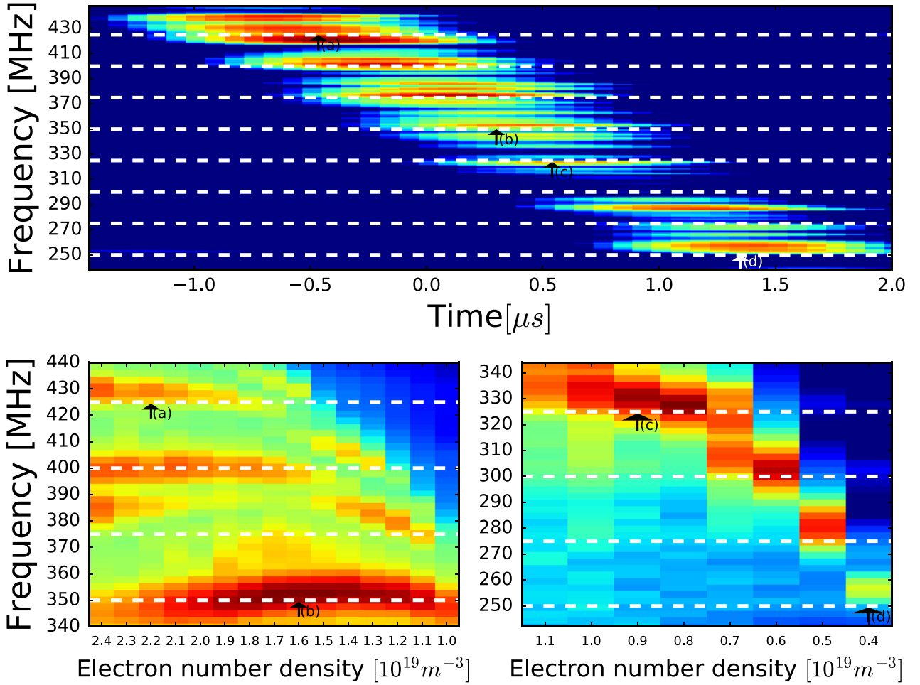
Figure 4. Top panel: experimentally-measured fast RF burst spectrogram from KSTAR plasma 11513 with B_0 = 1.99 T and average electron number density before the ELM crash \langle n_e \rangle = 2.6 \times 10^{19} \text{ m}^{-3} . Downward step-wise frequency chirping with f_{\text{cp}} \sim 25 MHz is apparent. Lower panels: as the lower panel of figure 3 but with B_z = B_{\text{cyc}} \approx 1.64 T.
