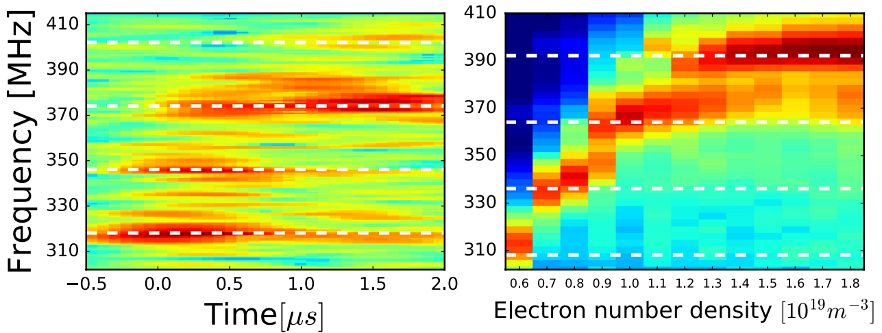
Figure 6. Left panel: experimentally-measured fast RF burst spectrogram from KSTAR plasma 11474 with B_0 = 2.27 T and \langle n_e \rangle = 2.5 \times 10^{19} \text{ m}^{-3} . Upward step-wise frequency chirping with f_{cp} \sim 28 MHz is apparent. Right panel: as the lower panel of figure 3 but with B_z = B_{cyc} \approx 1.84 T.
