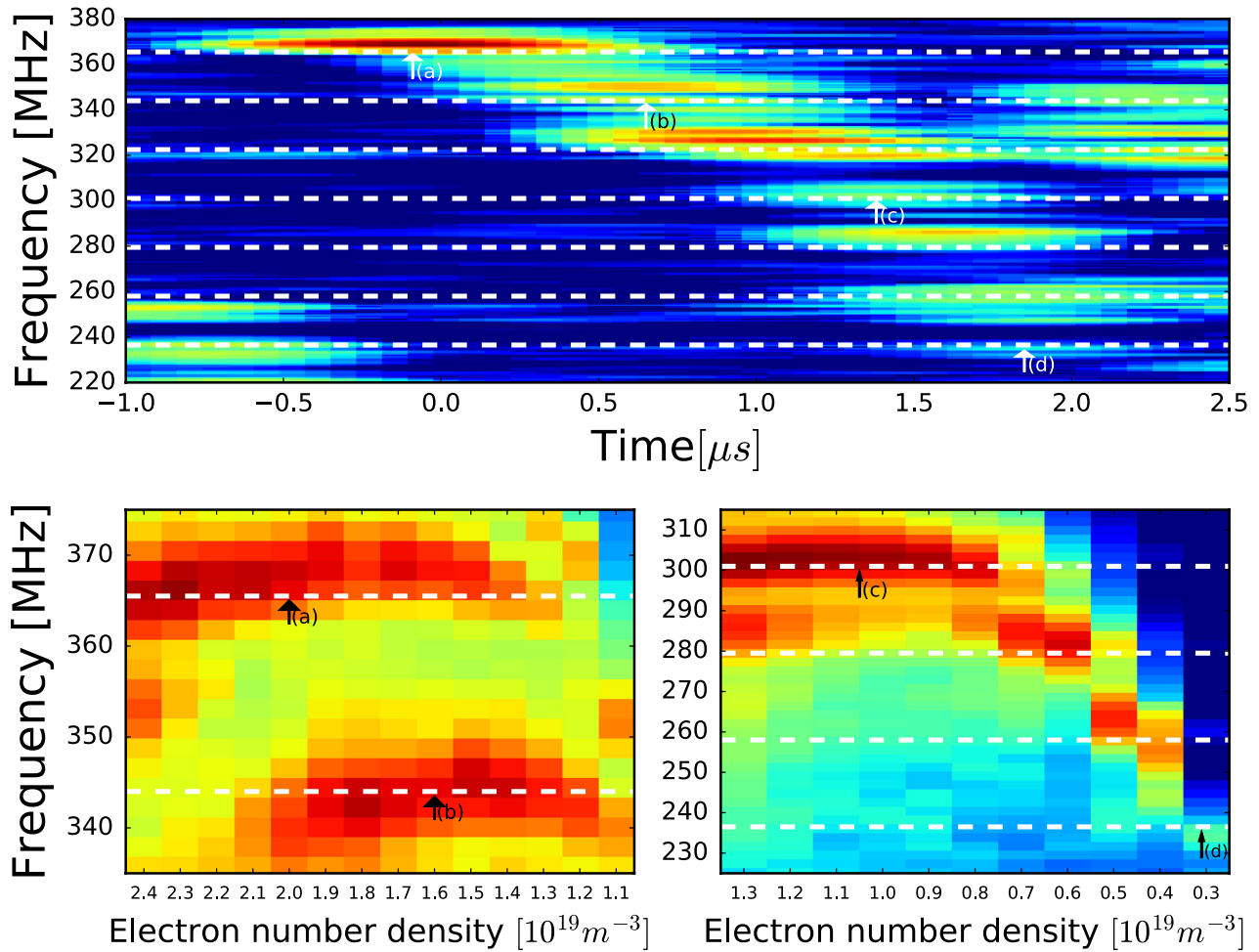
Figure 3. Top panel: experimentally-measured fast RF burst spectrogram from KSTAR plasma 11462 with B_0 = 1.7 T and average electron number density before the ELM crash \langle n_e \rangle = 2.5 \times 10^{19} \text{ m}^{-3} . Downward step-wise frequency chirping with proton cyclotron frequency f_{cp} \sim 21.5 \text{ MHz} is apparent. Lower panels: frequency versus electron number density plots for the nonlinear stage of MCI simulations where B_z = B_{cyc} \approx 1.41 T has been inferred from the data in the top panel. Shading indicates the \log_{10} of the spectral power in the fluctuating part of the B_z field component of each simulation.
