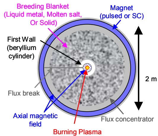
Figure 11. Midplane cross-section of FE with fissile-fusile breeding blanket.
