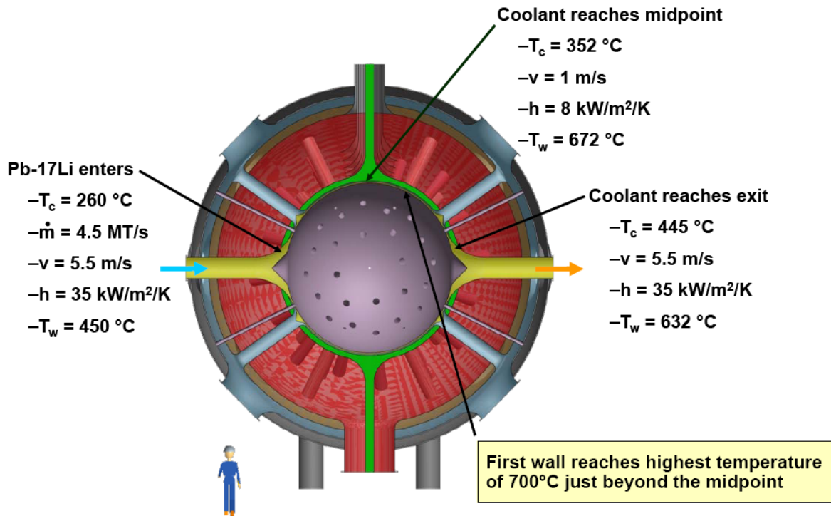
Figure 1. Cross-section through the proposed LIFE fusion-fission hybrid chamber.
