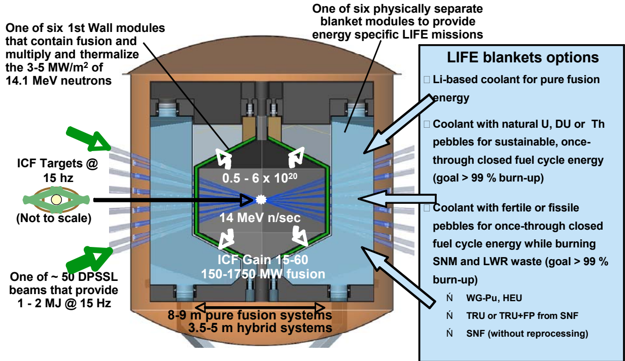
Figure 13. LIFE is designed to function at the first wall conditions and fusion confinement conditions (rR) required for a pure fusion system.
