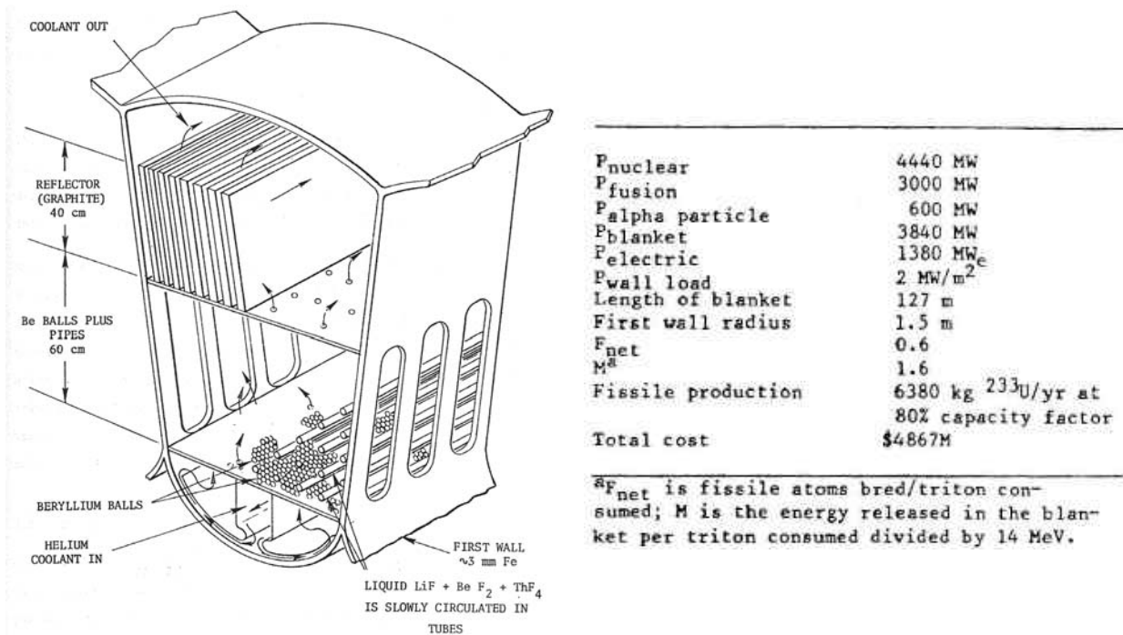
Figure 4. Fission-suppressed hybrid blanket based on beryllium pebbles and dissolved thorium in Flibe.
