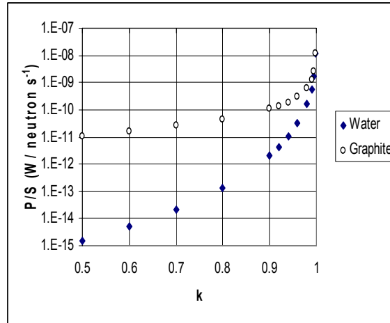
Figure 22. Power level per unit source (P/S) as a function of k_{\infty} for two different moderators.
